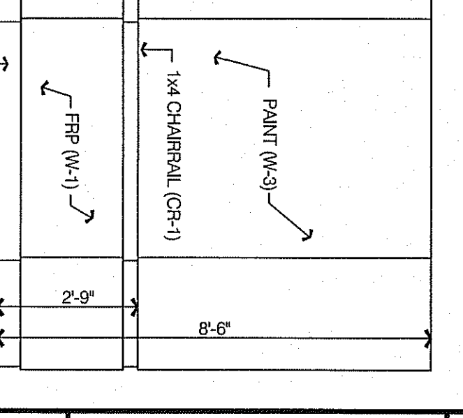
ROOM No. 121 CLASSROOM ELEVATIONS SCALE: 3/8" = 1'-0"
